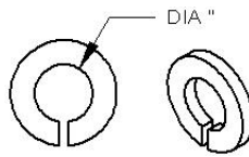
210-00117 WASHER, SPLIT LOCK 1/4" DIA.
