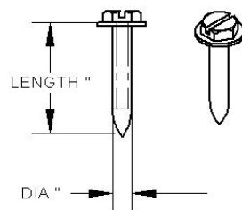
210-00273 LAG BOLT W/WASHER 1/2" DIA. X 1 1/2" LONG
