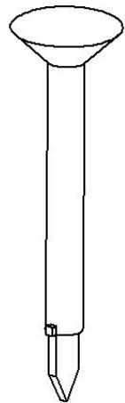
210-00131 SCREW, TORX FLAT HEAD SELF DRILL 14 X 2 3/4"
