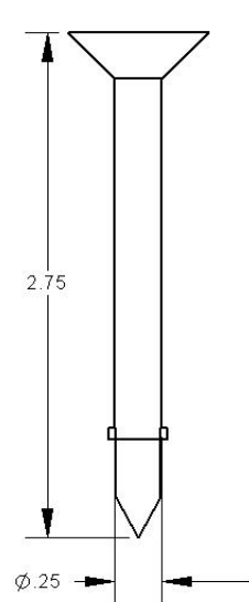
210-00131 SCREW, TORX FLAT HEAD SELF DRILL 14 X 2 3/4"
