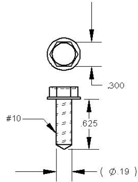
210-00057-NA SCREW, #10 X 5/8 HEX WASHER HEAD
