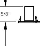
210-00173 NUT 5/16" - 18 T-NUT W/ 5/8" BARREL LENGTH
