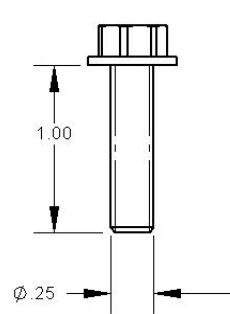
210-00121 SCREW W/WASHER 1/4" - 14 X 1 W/MILLED PNT
