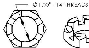
210-00062 NUT, SLOTTED JAM (CASTLE NUT) 1" - 14
