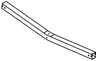
100-00011-GL 100-00011-WH CROSSMEMBER 3 X 3 X 66.25"
