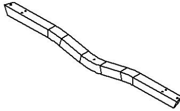
100-02160-AL CROSSMEMBER - FRONT 3 X 3 X 61.03"
