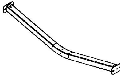
300-01066-BL 300-01066-GL 300-01066-WH CROSS MEMBER WELDMENT 3 X 3 X 73.5"
