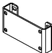
100-02205-GL 100-02205-ZN SPACER CHANNEL 5" X 6 3/4"
